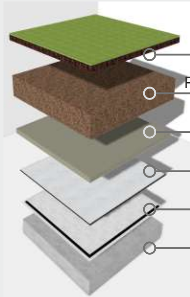
Lawn Plantation in 175 mm thickness
