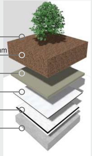
Shrubs Plantation in 200 mm
